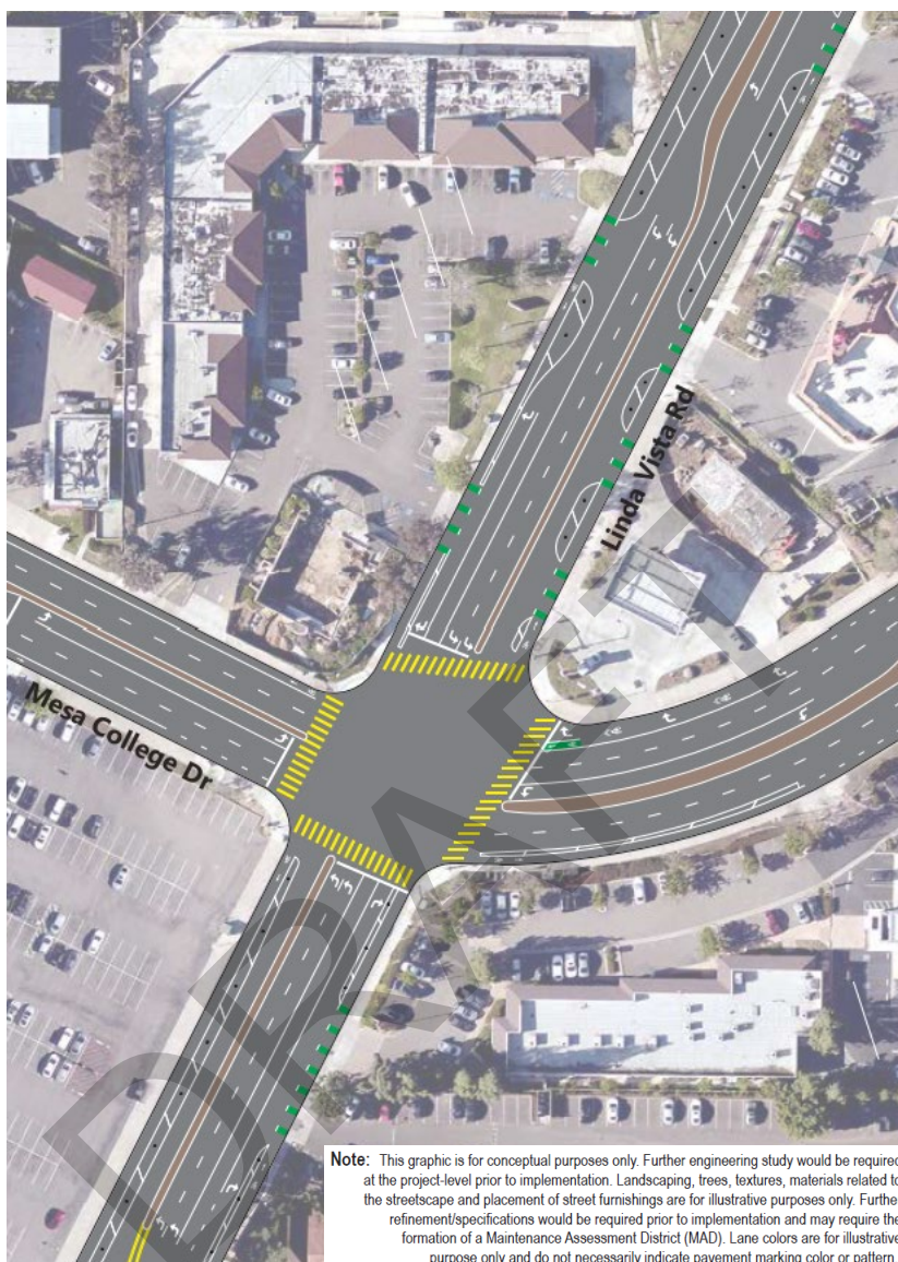
Figure 14 – Conceptual Improvements at Intersection Linda Vista Road and Mesa College Drive
